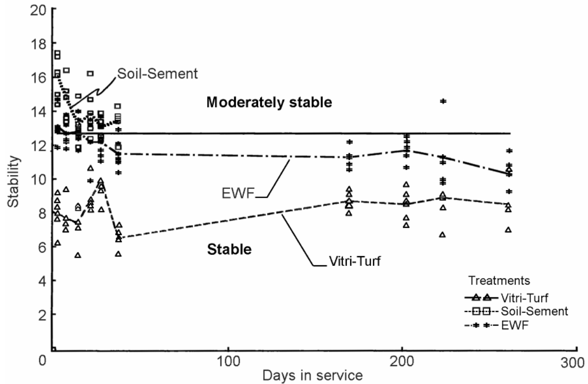
Figure 13—Stability of playground surface, as measured by rotational penetrometer, over 9-month installation.
