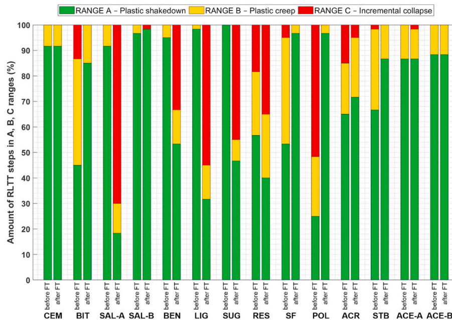
Fig. 11. Classification of each RLTT step based on the permanent deformations measured before and after FT cycles.
