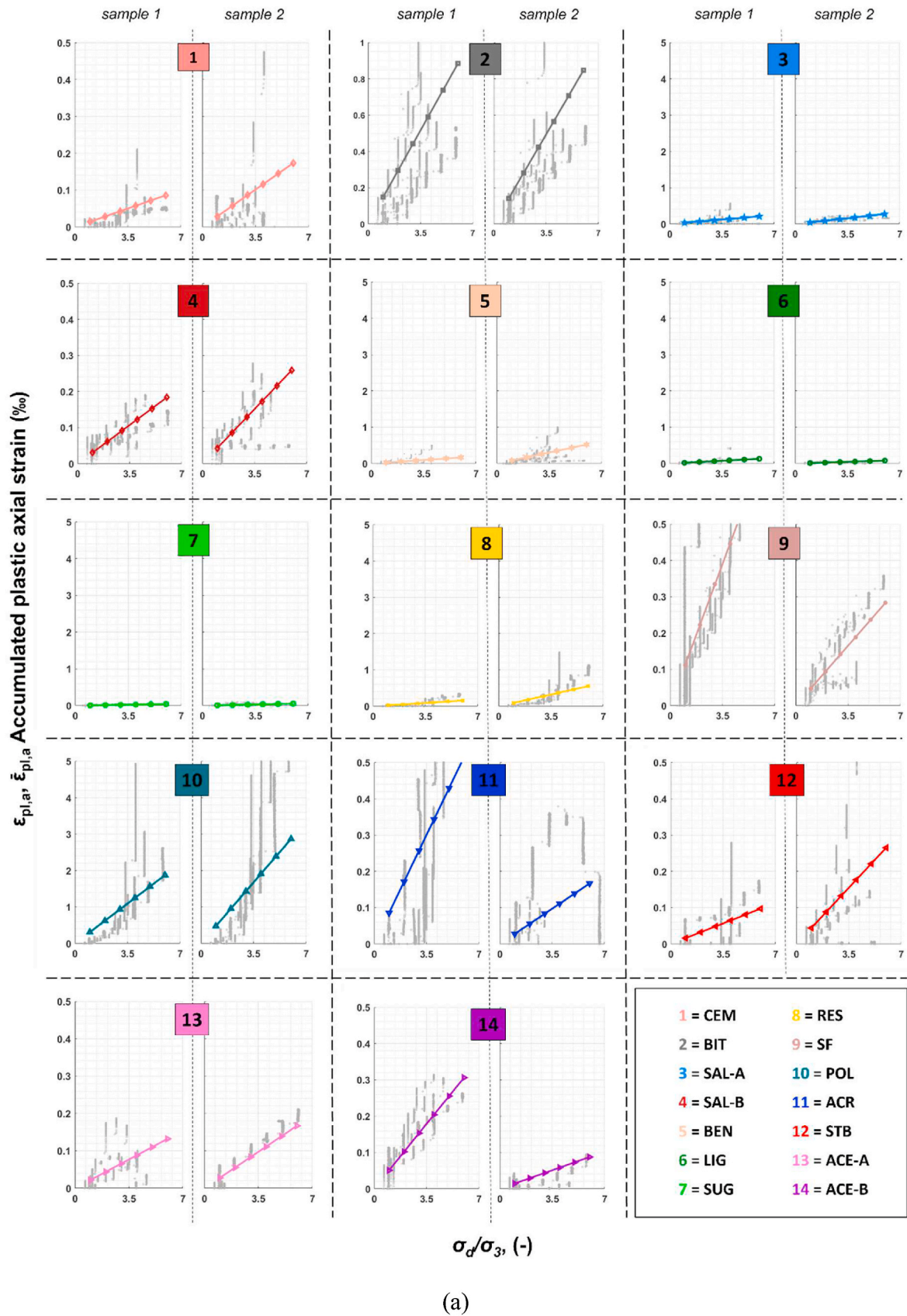
Fig. 9. Experimental data of accumulated plastic axial strain \epsilon_{pl,a} (grey dots) and average calculated trends \bar{\epsilon}_{pl,a} (colored solid lines) before (a) and after (b) 10 FT cycles.
