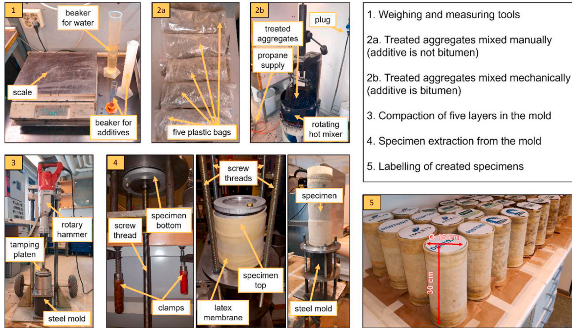
Fig. 2. Main steps to create RLTT samples.
