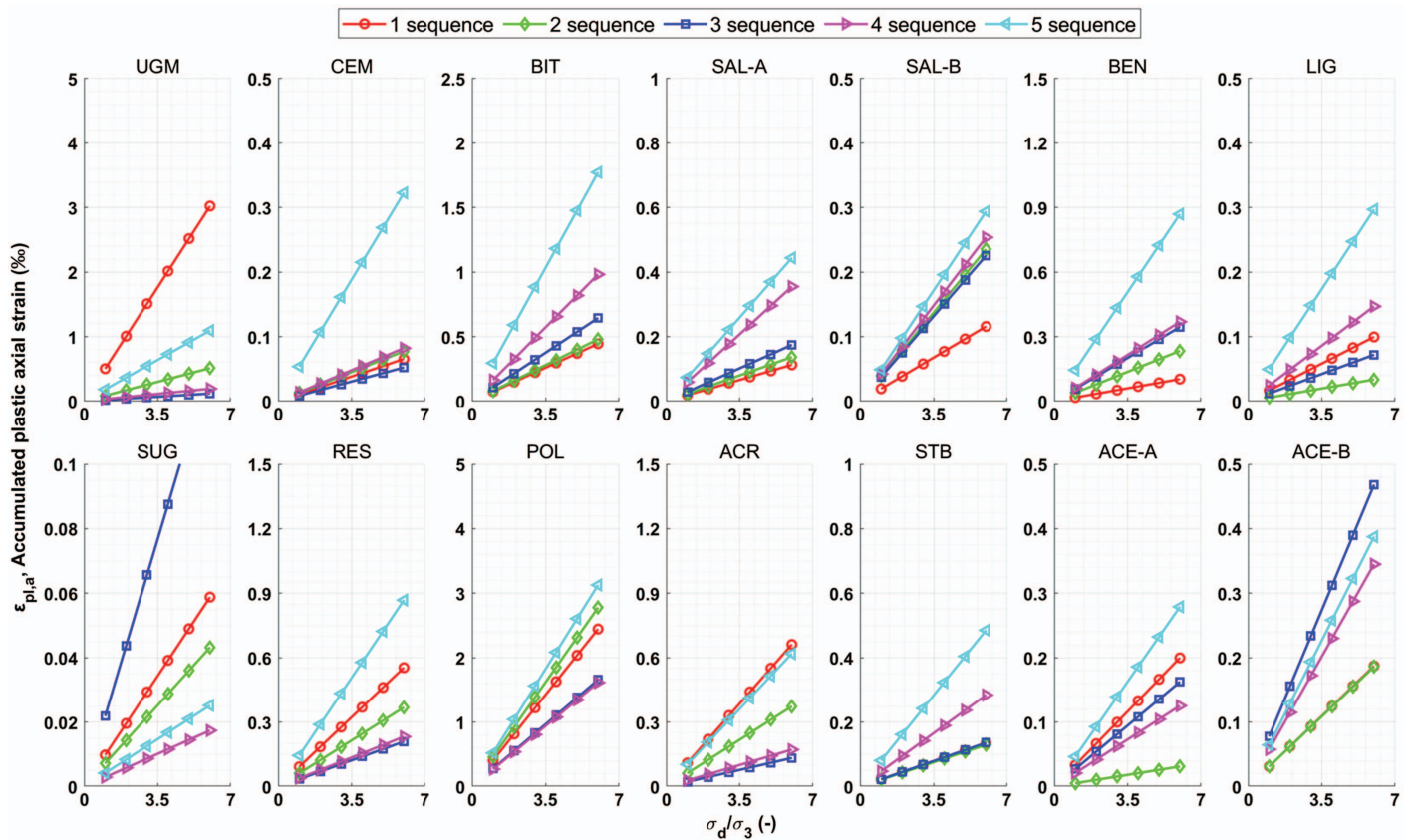
Fig. 8. (Color) Accumulated plastic axial strain \epsilon_{pl,a} modeled according to Hyde model.
