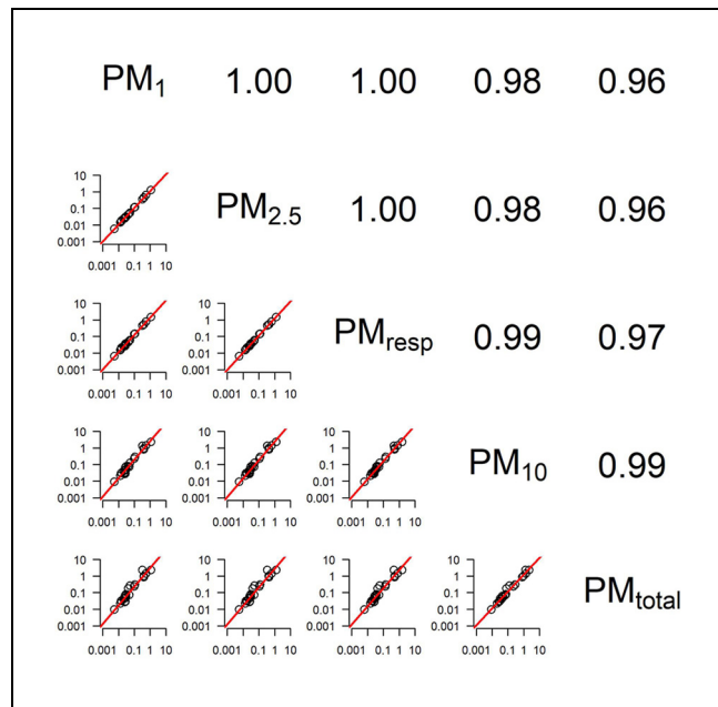
Figure 4. Correlations between five measures of dust production. Variables and associated dust size ranges are as follows: PM 1 (0.1 to 1.0 \mu m); PM 2.5 (0.1 to 2.5 \mu m); PM resp (0.1 to 4.0 \mu m); PM 10 (0.1 to 10 \mu m); and PM total (0.1 to 15 \mu m). Numbers in panels above the diagonal show Pearson product moment correlation coefficient ( r ). Red lines show linear relationship between the variables. Note that all axes are on a log 10 scale.
