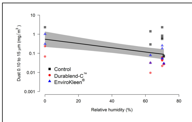
Figure 5. Total dust production ( PM_{total} ; 0.10 to 15 \mu m ) decreased with increasing relative humidity (%) on untreated and treated road segments. Shaded area indicates 95% confidence interval. Note that the y-axis scale is logarithmic. Points represent samples taken on a particular road segment on a particular date.
